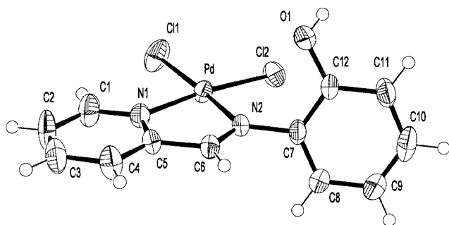
Figure 1. Perspective view of molecule 1c ·THF; thermal ellipsoids are drawn at the 50% probability level; the solvent has been omitted
