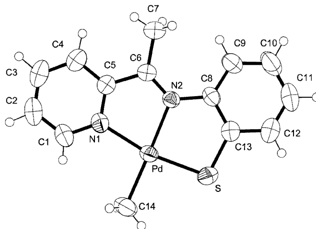
Figure 4. Perspective view of molecule 2b ; thermal ellipsoids are drawn at the 50% probability level
