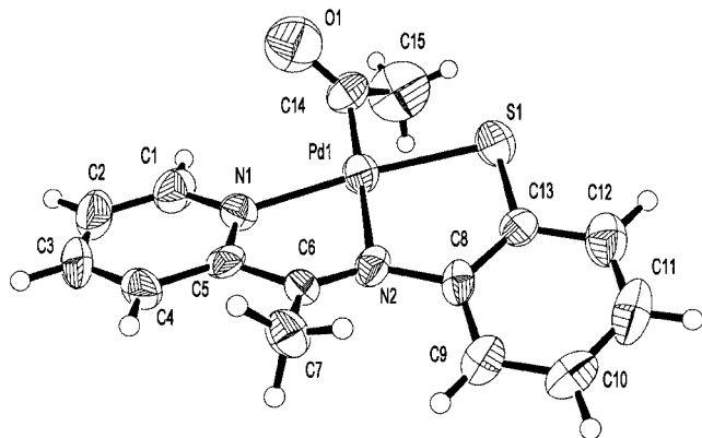
Figure 5. Perspective view of one of the two independent molecules in the crystal structure of 2c ·1/2CH 2 Cl 2 ; thermal ellipsoids are drawn at the 50% probability level; the solvent has been omitted
