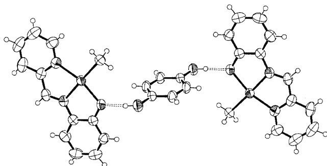
Figure 3. Molecular assembly through hydrogen bonds in the cocrystallization of 1b with hydroxyquinone
